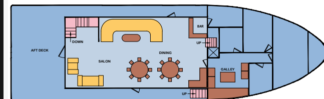
MAIN DECK
